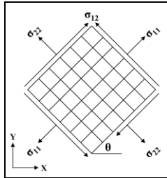
Figure 4: Local and global stress components (stress transformation)
